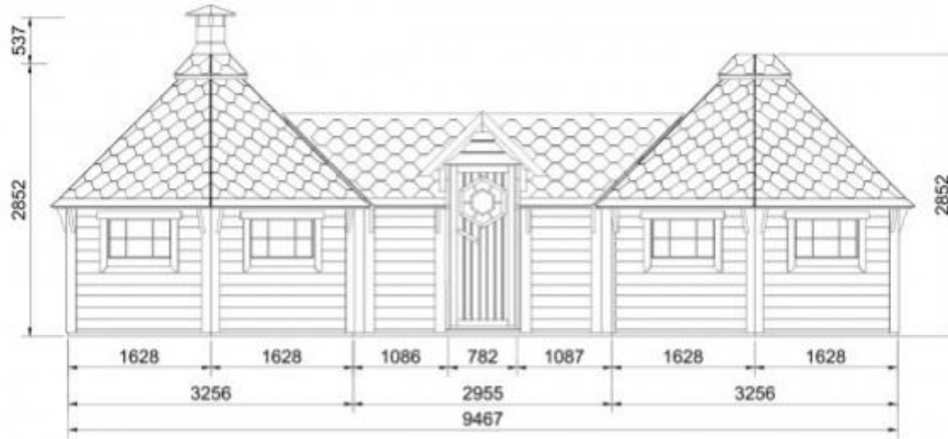
Back view
